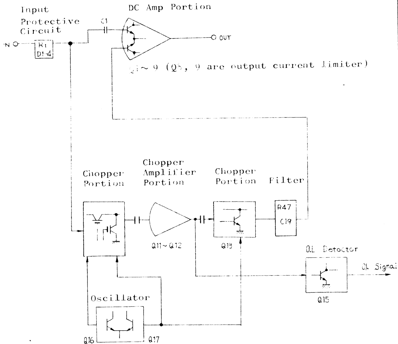
Fig. 5.1.1 Block Diagram of Quad DC Amplifier
