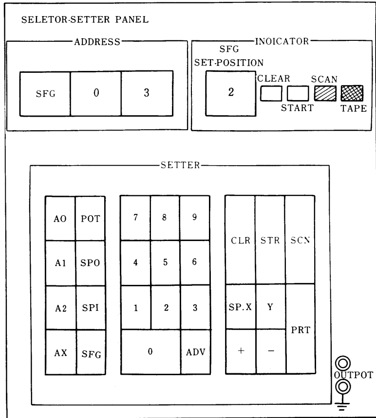
SELECTOR-SETTER PANEL LAYOUT
